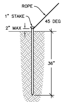
STAKE DETAIL
