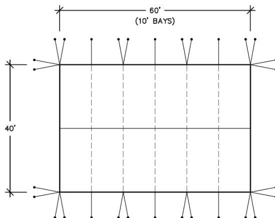
STAKING PLAN
